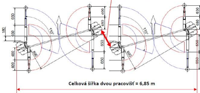
Zvedák Consul Z235 Comfort
